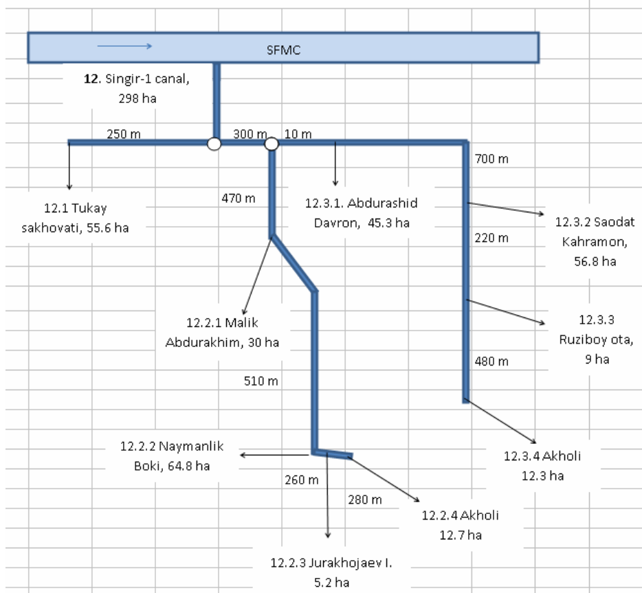
Figure 1. Linear network of the Singir-1 canal
